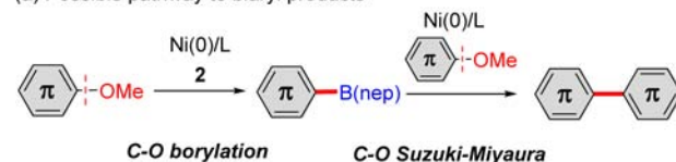
Scheme 4. Possible Pathway and Ligand Effect
